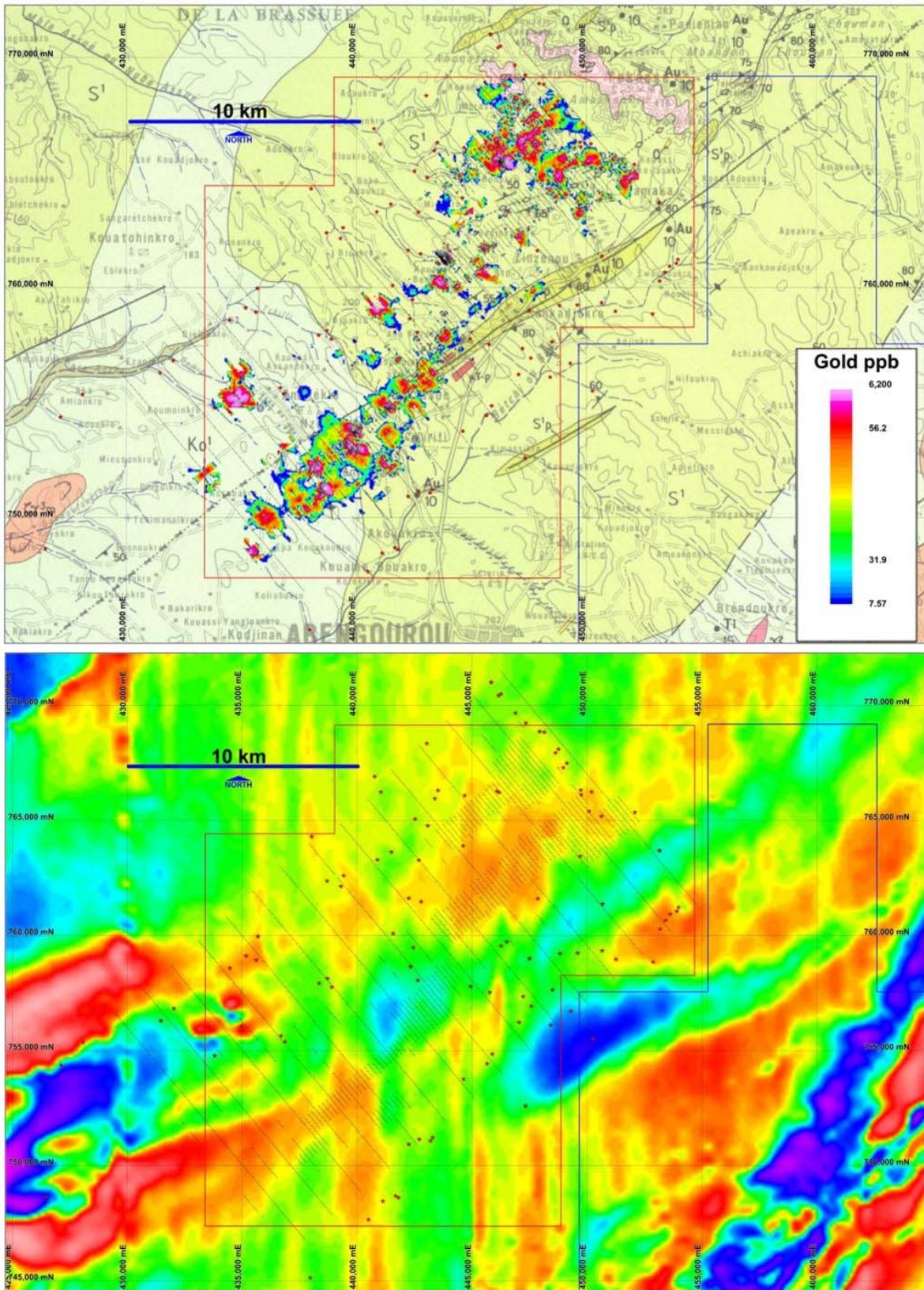
Figure 2: Amélékia Legacy Gold Soil Geochemistry grid over Government Geology (top) and Soil Locations over Government Aeromagnetics (bottom). Both maps at same scale.
