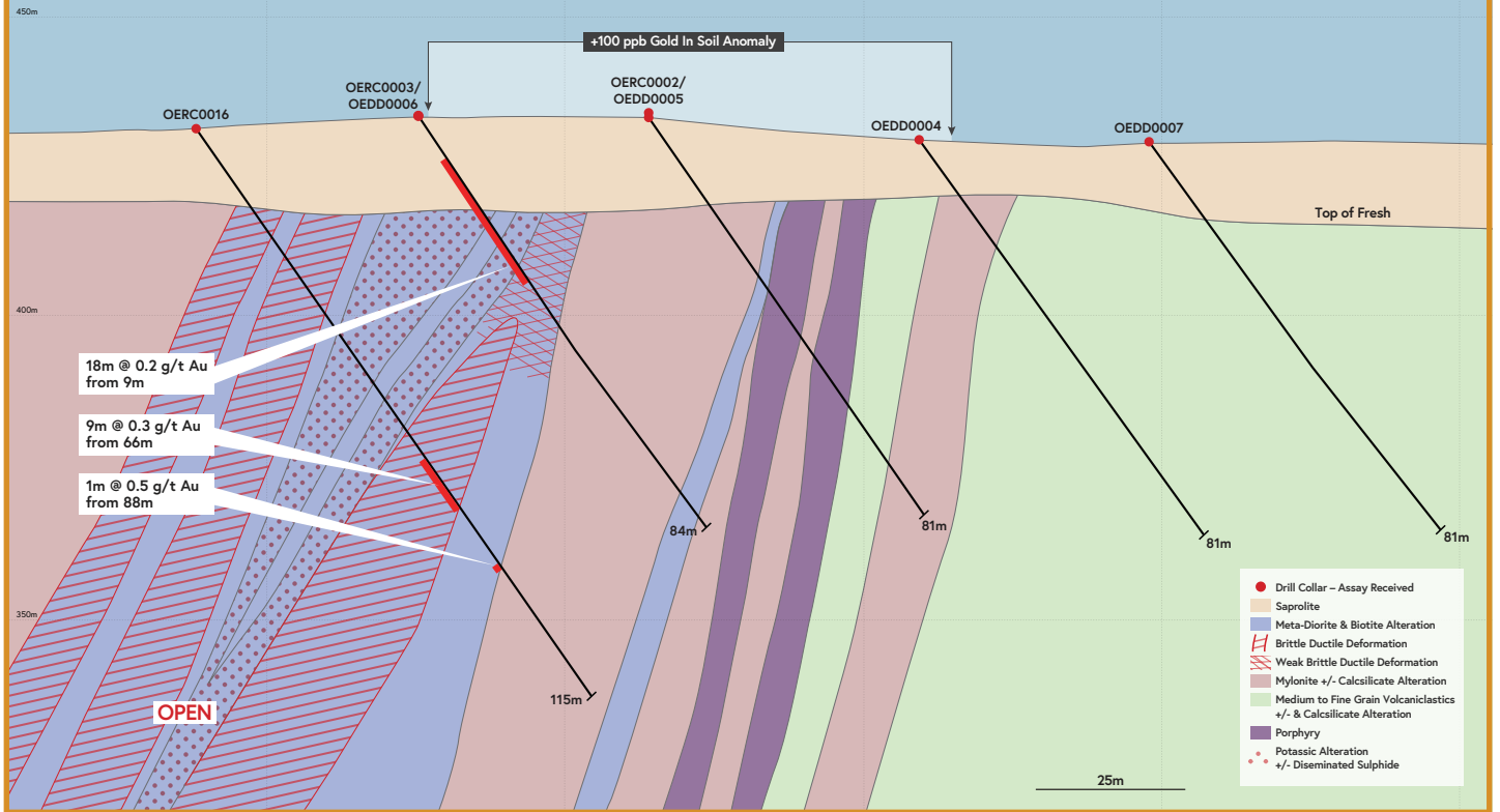
Cross Section 3 – Looking Northwest
