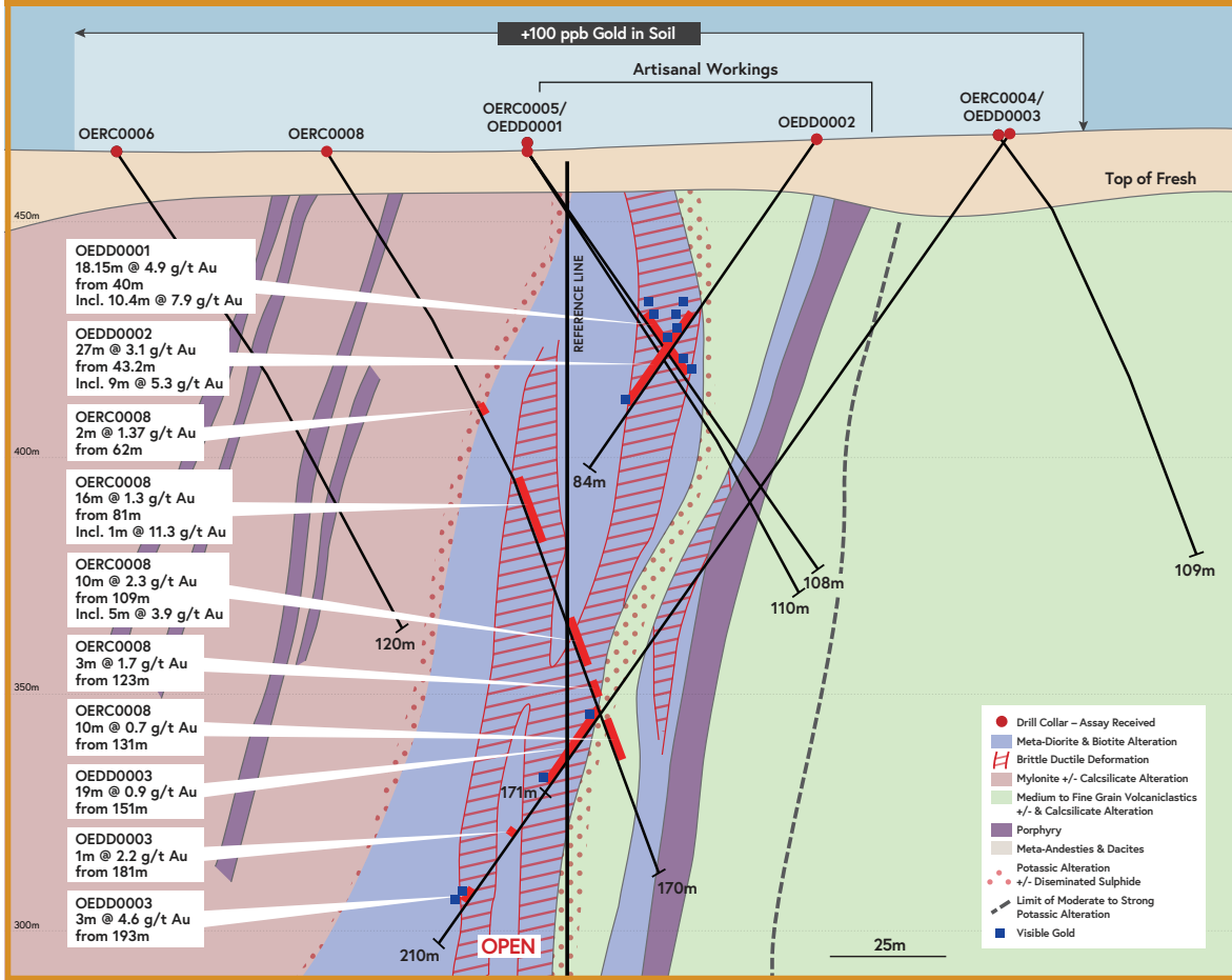
Cross Section 2 – Looking Northwest
