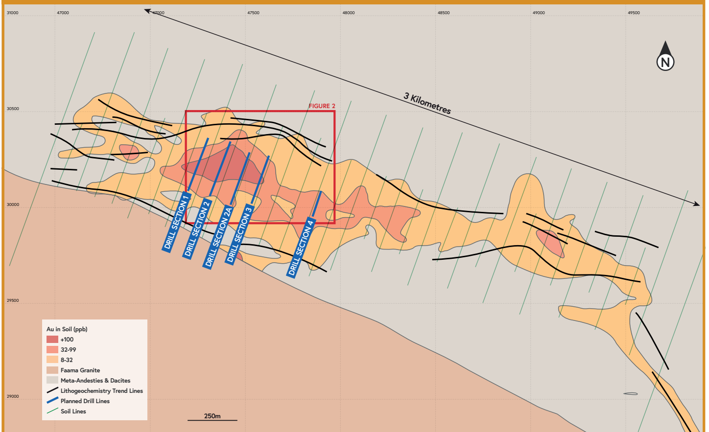
Empire – Soil Geochemistry and RC/DD Drill Lines
